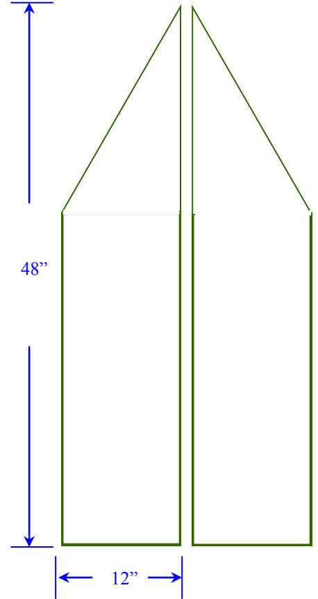
3.5" - 3.75" Outside Corner
